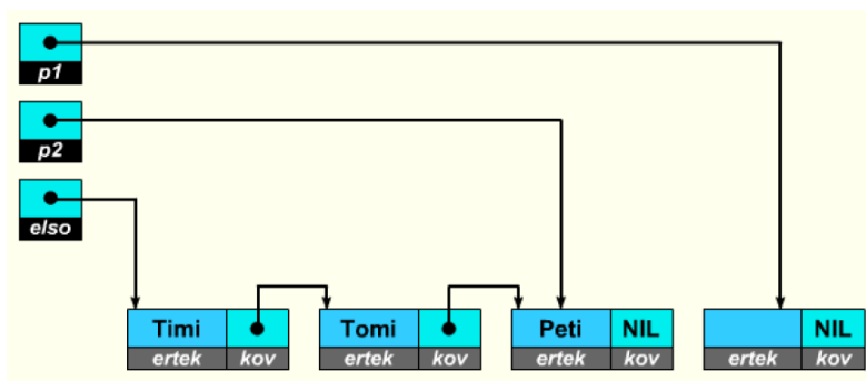
Figure 9. Visualization of singly linked list (Végh, 2017)
