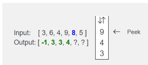
Figure 7. Visualization of stack for the example task
