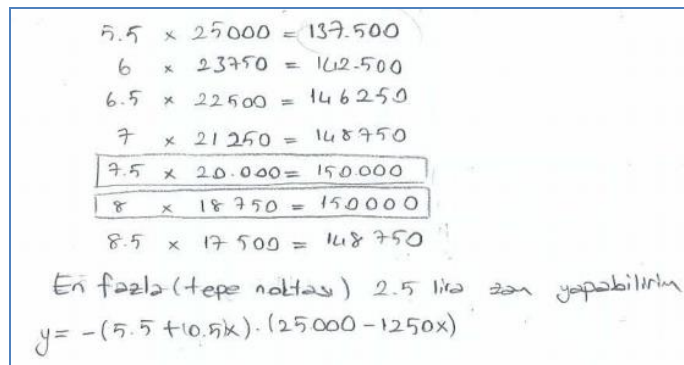
Figure 4. Group-4's Solution
