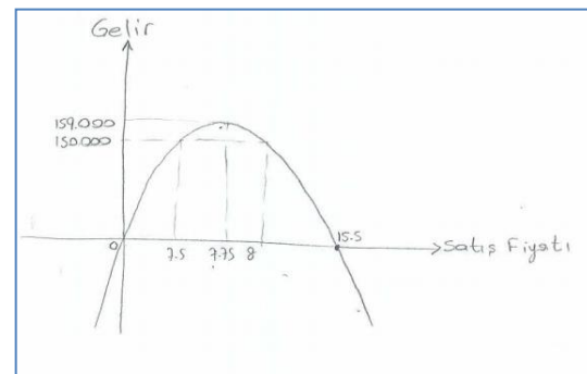
Figure 6. Group-8's Graph
