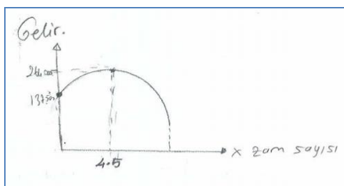
Figure 7. Group-7's Graph
